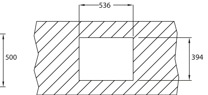
Hueco para bajo encimera Fitting hole for undermounted sink
